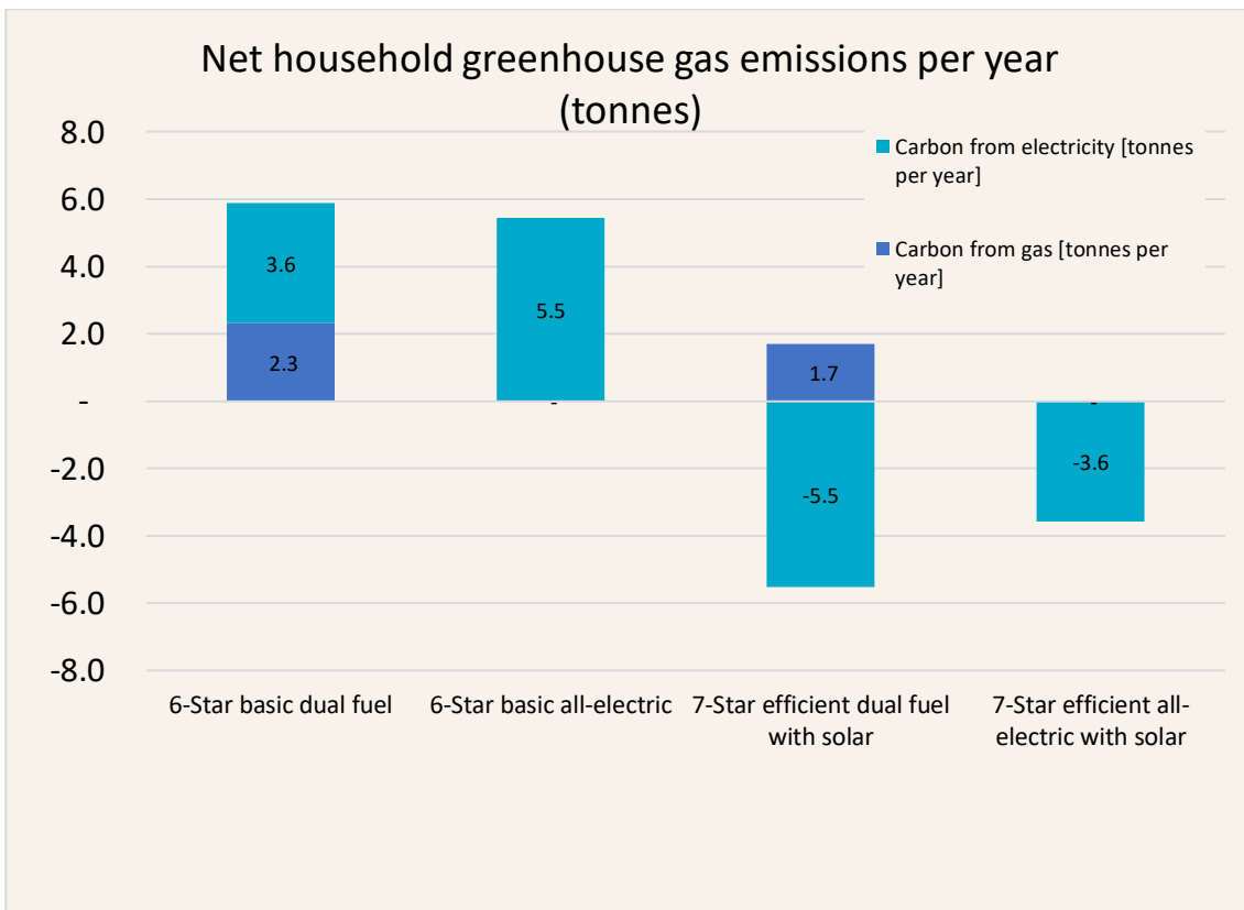
Figure 7. Net household GHG emissions
